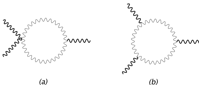
Figure 4: Gauge one-loop three-point functions from vector loop.
