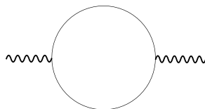
Figure 1: Gauge one-loop two-point functions from chiral loop.
