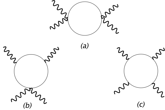
Figure 3: One-loop four-point functions with chiral loop.
