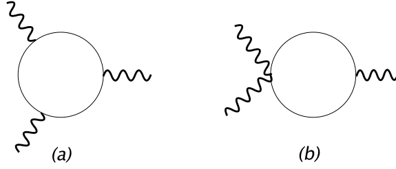
Figure 2: One-loop three-point functions with chiral loop.
